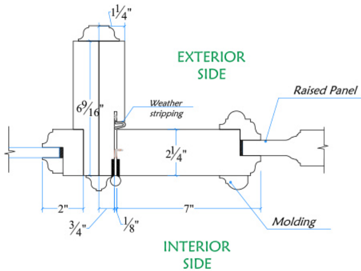
Stile Detail/Hinge
